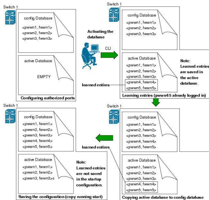
Figure 24 : Port Security Database Scenarios
